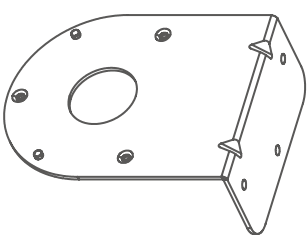
Support mural (×1)
